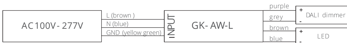
DALI dimming connection diagram
