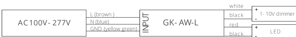
1-10V dimming connection diagram
